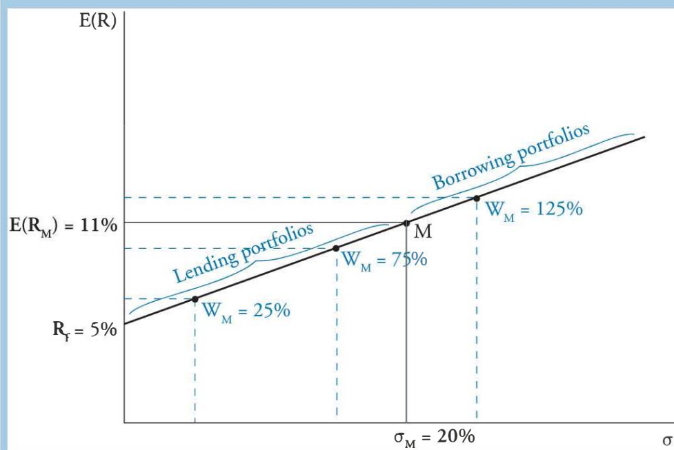
Figure 4: Borrowing and Lending Portfolios
